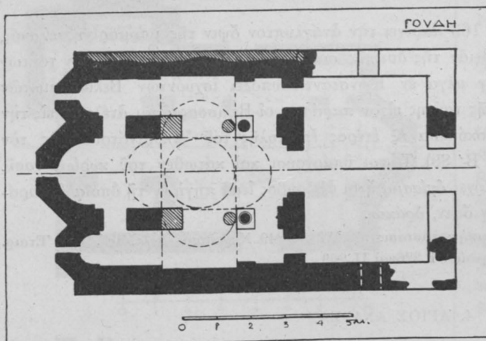
Εἰκ. 165. Κάτοψις τοῦ ναοῦ τῆς Παναγίας Γουδῆ.
